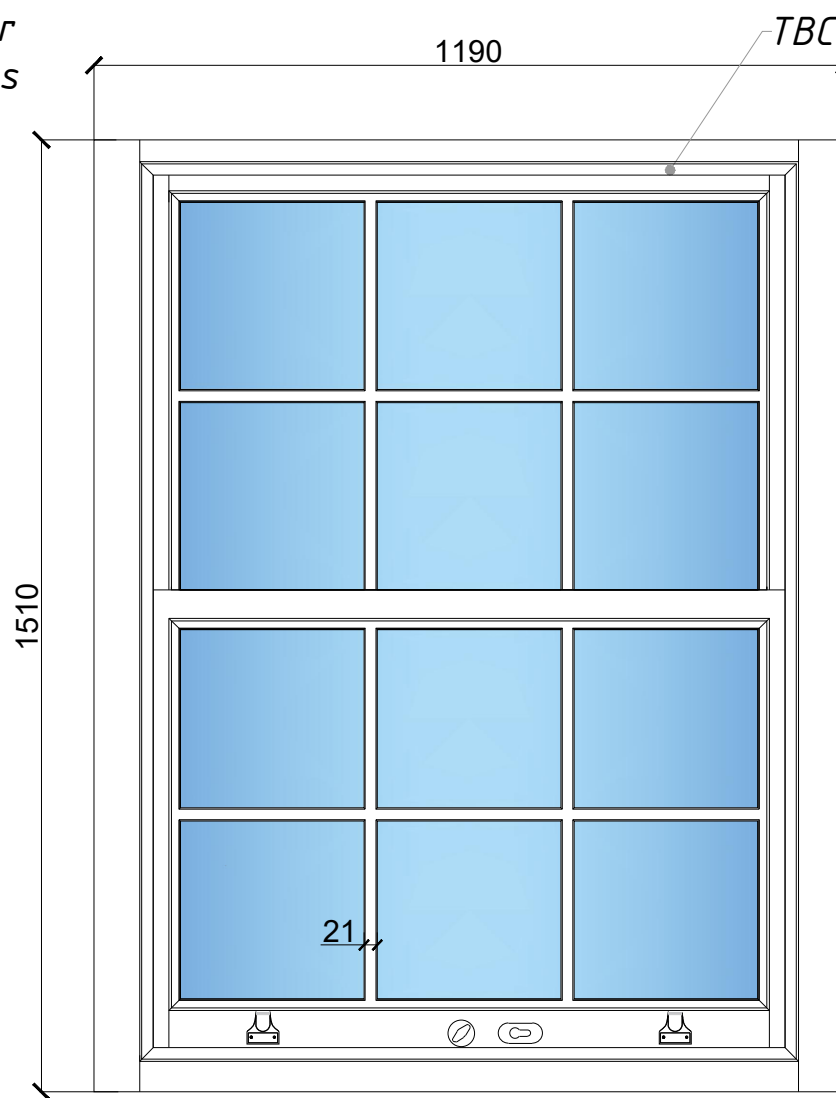
Internal elevation
