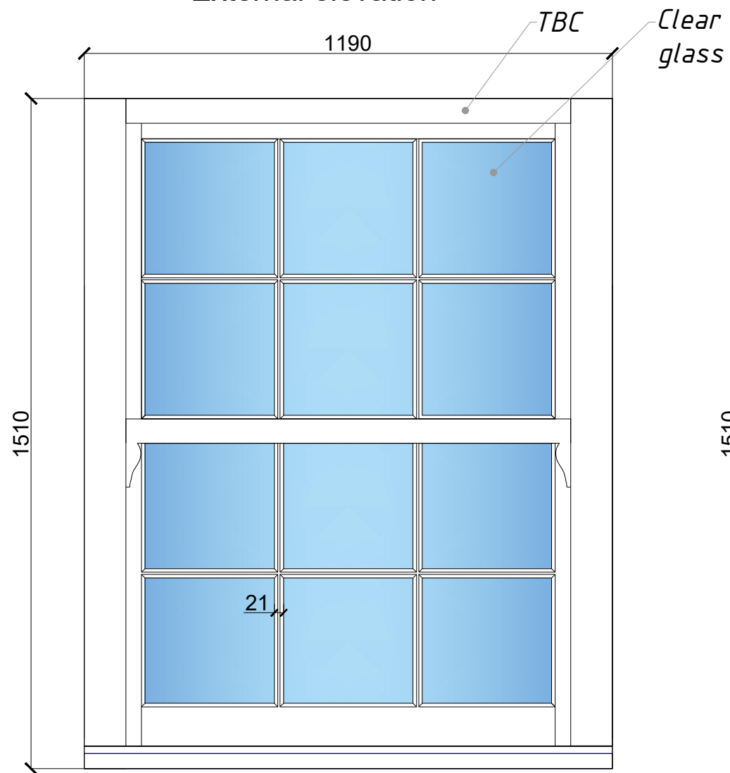
External elevation
